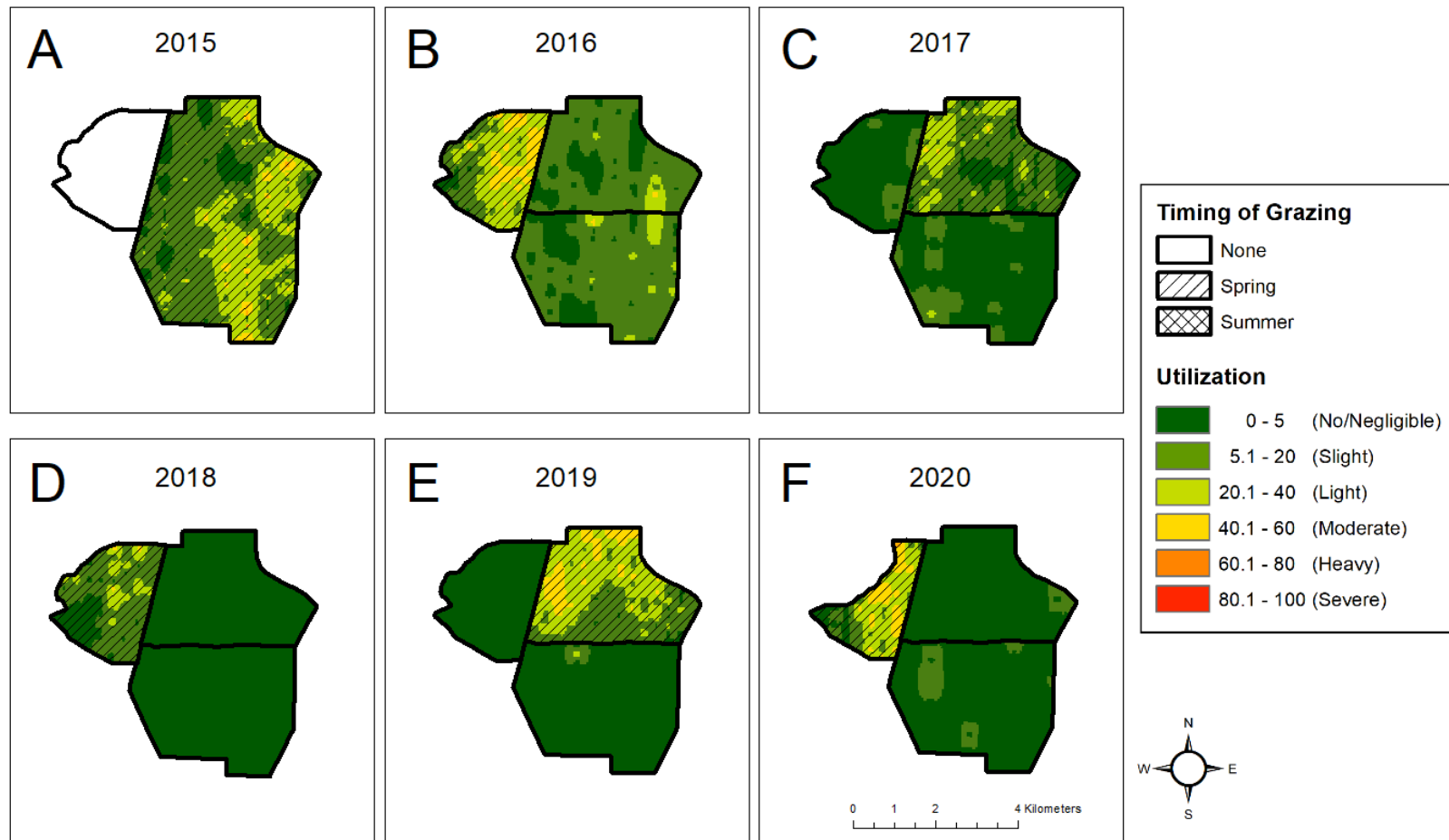
Figure 13. Pattern use mapping based on landscape appearance transects at Jim Sage, Idaho 2015-2020.
