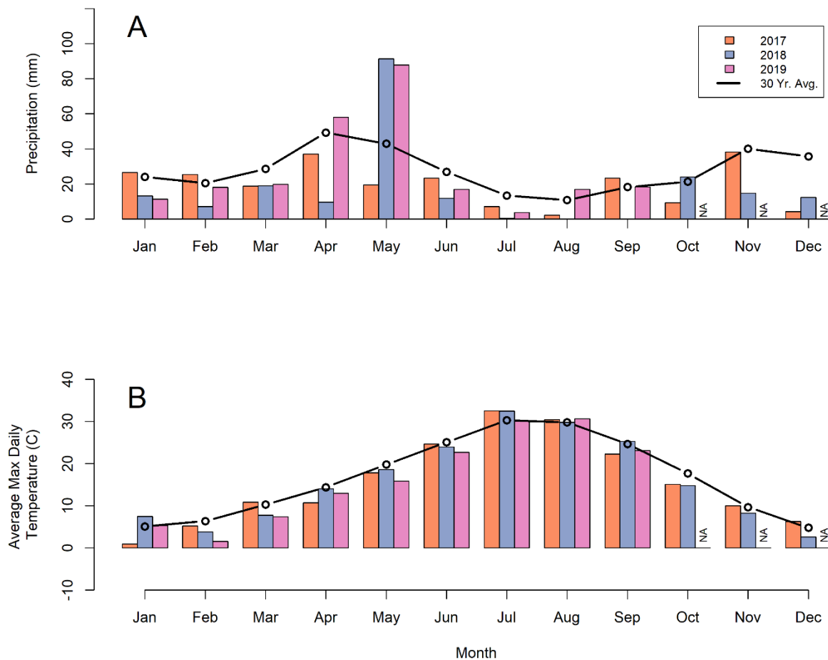
Figure 4. Monthly precipitation totals (A) and average max daily temperature by month (B) with 30-year average (dark line) at Sheep Creek, Idaho 2017-2019.
